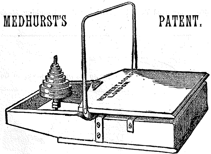
No. 202.—Improved Lever Weighing Machine for Coals, and Field Use.
