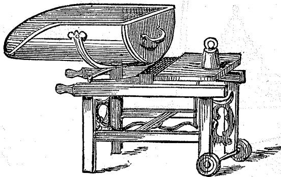
No. 204.—Retail Coal Machine.
