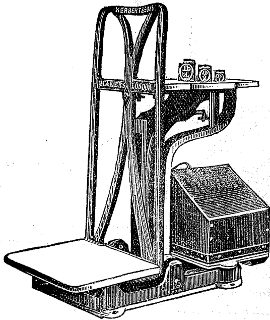
No. 203.—Improved Patent Curvilinear Coal Weighing Machine.
