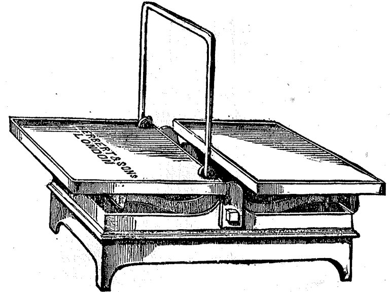
No. 201.—Specially constructed for carrying under Coal Vans.
