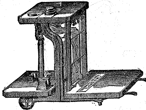
No. 186.—Improved Low Weighing Machine, Extra Strong, suitable for Wholesale Houses and Wharf Work.
