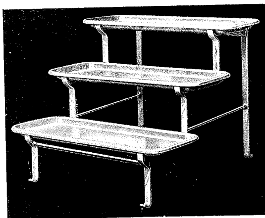
No. 677. 3 Tier as illustrated with Enamelled Dishes. Size of Dishes 18" x 7" Height of Stand 14 1/2" Depth of Stand 18" Price complete 15/9
