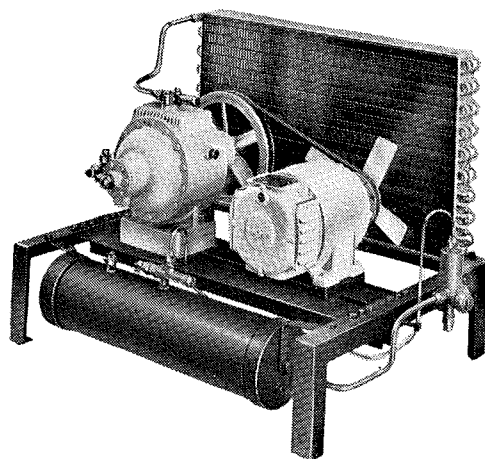
Superfrigor Rotary Unit with Duo-Condensers.
