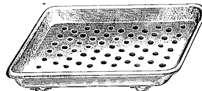
No. 64. Bottom perforated 1/4" holes. 1/2" small feet at each corner.
