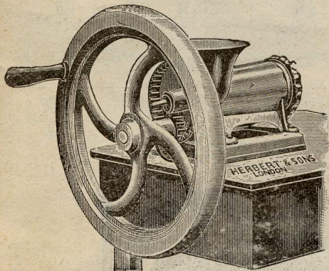
No. 1 GEARING.
