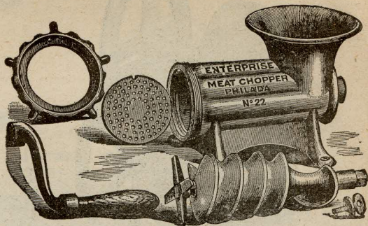
SHOWING MACHINE TAKEN APART.
