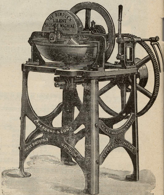
No. 4—With Five Knives.
